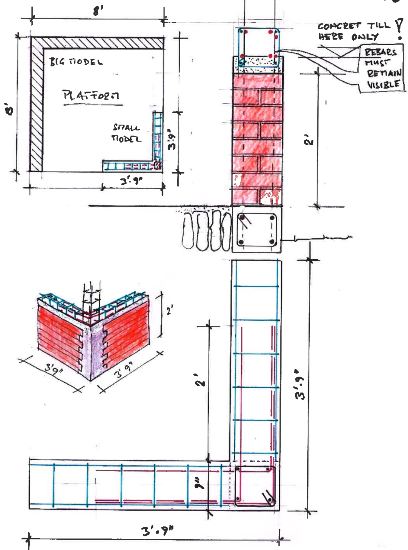
SECTIONED RED MODEL "CONFINED MASONRY" FLASH + BOND BEAM MODEL
