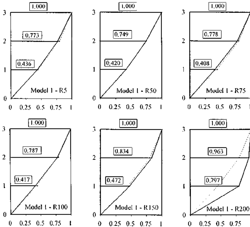
Figure 7. First natural vibration mode shapes
